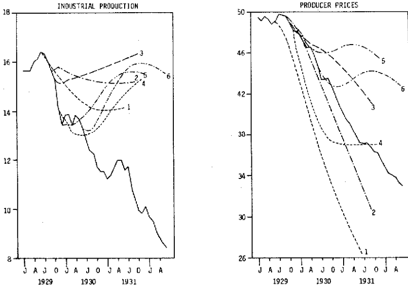
FIGURE 7. ACTUAL AND FORECAST VALUES: MODERN DATA, SAMPLE BEGINS MAY 1908. Note: System includes industrial production (Babson), producer prices, three-month time loan rate, stock prices, and M2. Solid lines are actual data. Dashed lines are forecasts conditional on data through June 1929 (1), September 1929 (2), October 1929 (3), November 1929 (4), December 1929 (5), and June 1930 (6).
